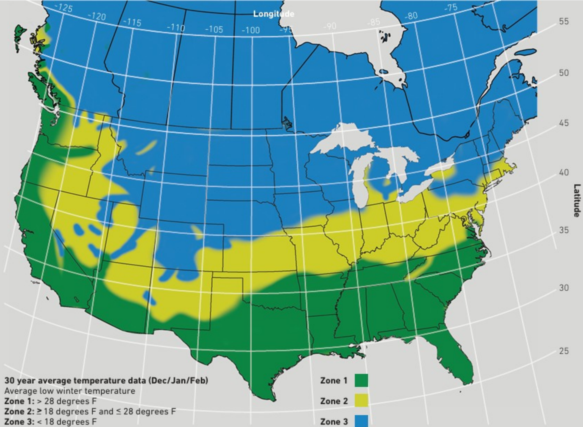
Figure 2.1.2-1 | Climate Exposure Zones for Roadway Applications per Table 2.1.2-1
