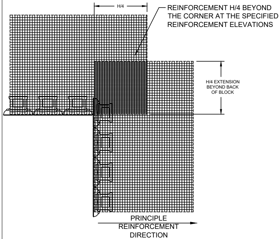
GEOGRID LAYOUT
