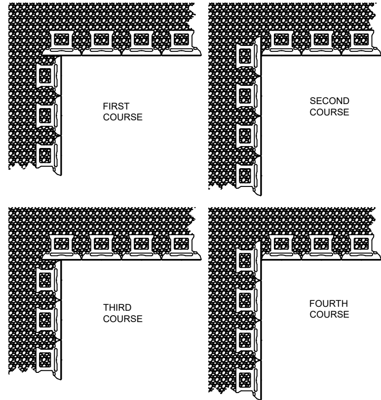
BLOCK LAYOUT
