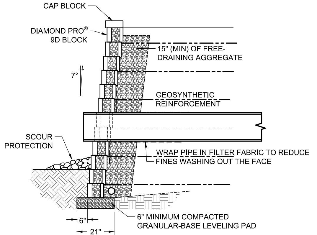
SECTION VIEW
