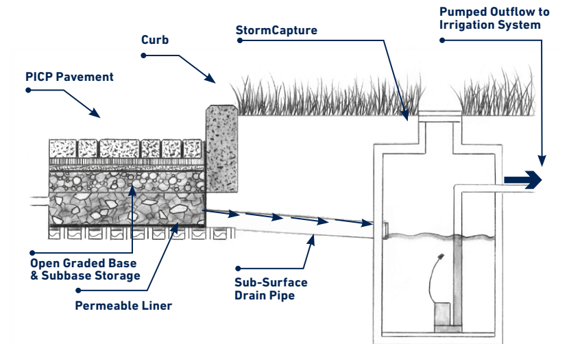
Water Harvesting Using PICP
