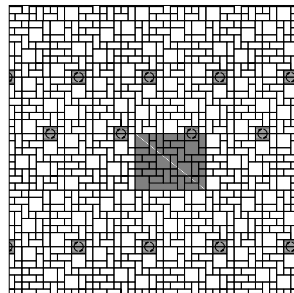
RUNNING BOND (MECHANICAL) 4 1/2 X 4 1/2 (22%), 4 1/2 X 9 (25%), 9 X 9 (53%)
