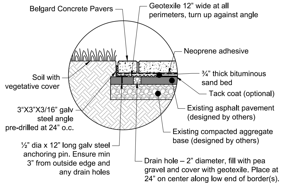
EDGE RESTRAINT - BITUMINOUS SET ON EXISTING ASPHALT BASE
