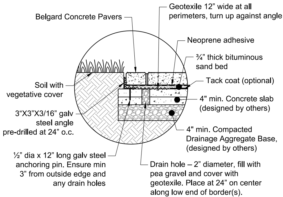
EDGE RESTRAINT - BITUMINOUS SET ON CONCRETE BASE
