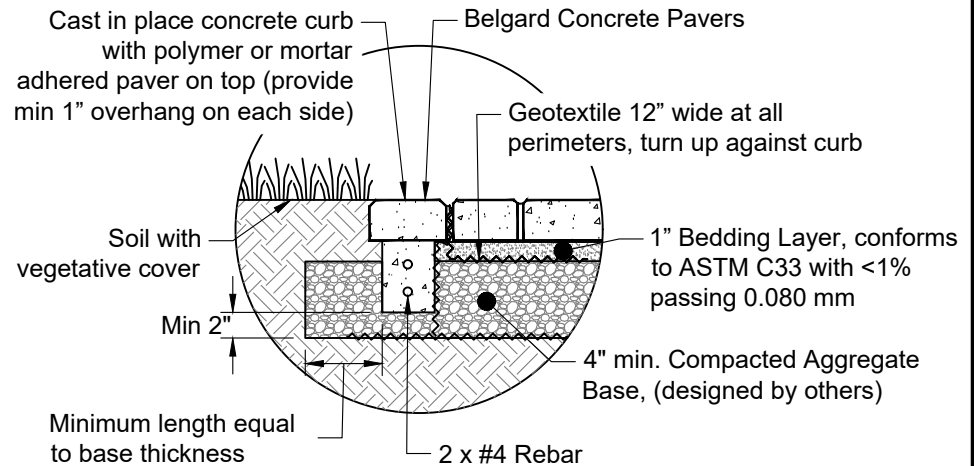
EDGE RESTRAINT - SAND SET ON AGGREGATE BASE
