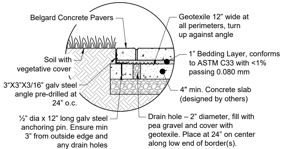
EDGE RESTRAINT - SAND SET ON CONCRETE BASE
