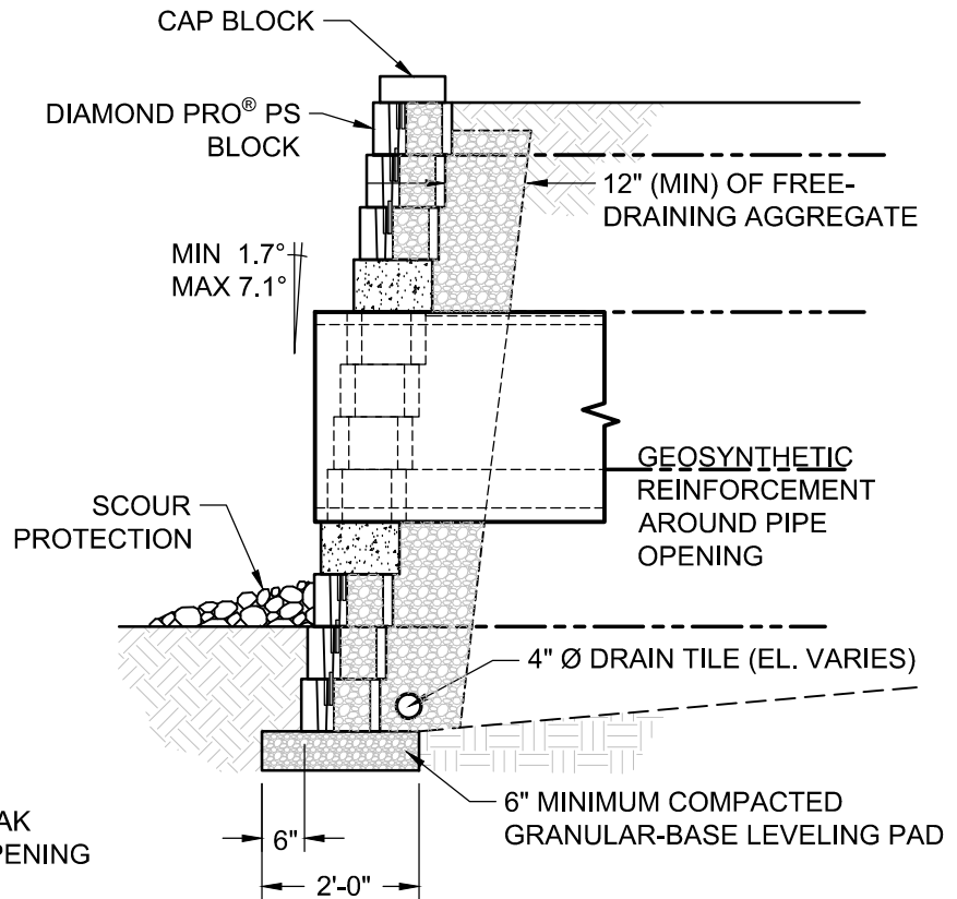
SECTION VIEW
