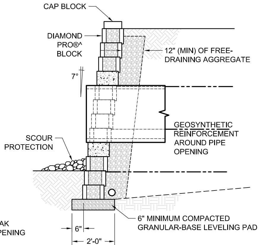
SECTION VIEW
