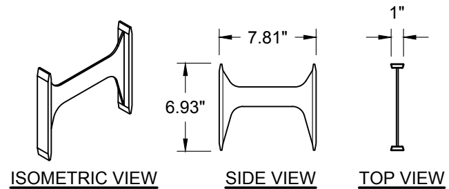
CONNECTOR
